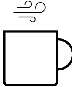
Forced Convection
