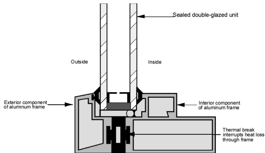
Diagram 5-2. A thermal break in an aluminum frame.
