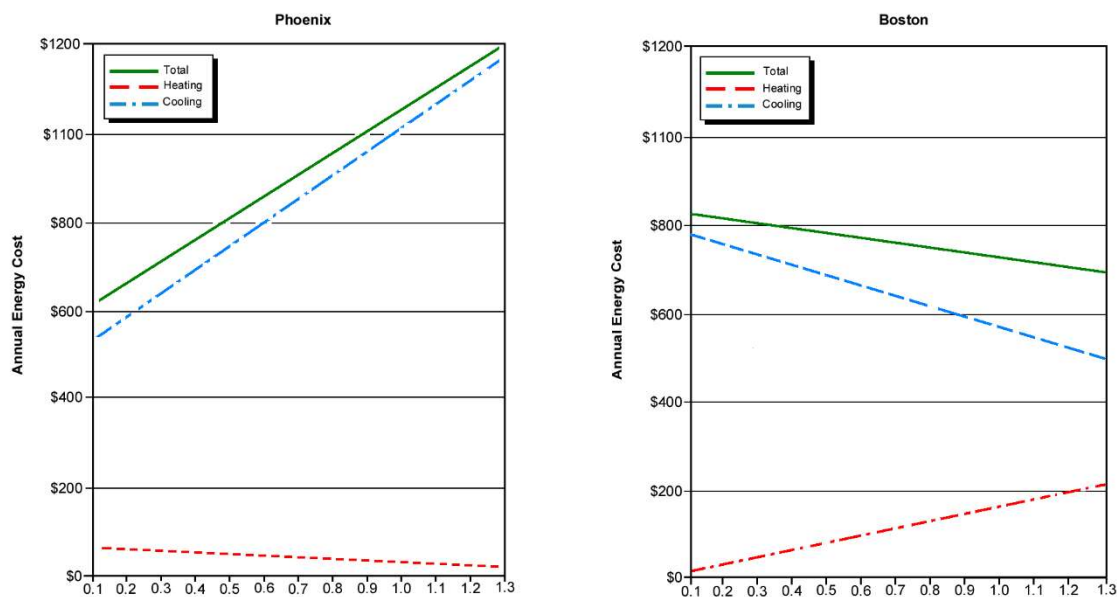
Diagram 3.5. Effect of solar heat gain coefficient (SHGC) on annual energy costs.
